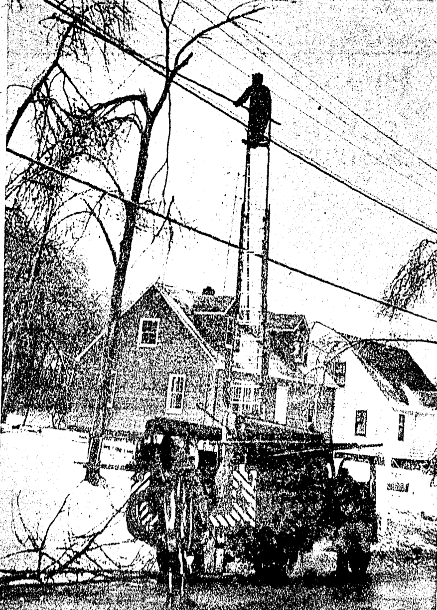
Several crews of workers worked steadily since Friday trimming and removing broken branches and replacing power lines damaged in the recent storm. One of the crews is shown wearing slickers against the wet and preparing to remove a limb fouled in the power lines.
